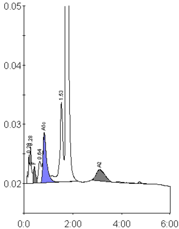
Peak table - ID: 10362515
